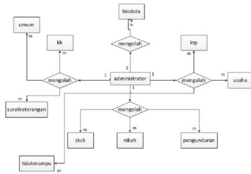
Gambar 1. Rancangan Entity Relationship Diagram Sistem Administrasi Surat
